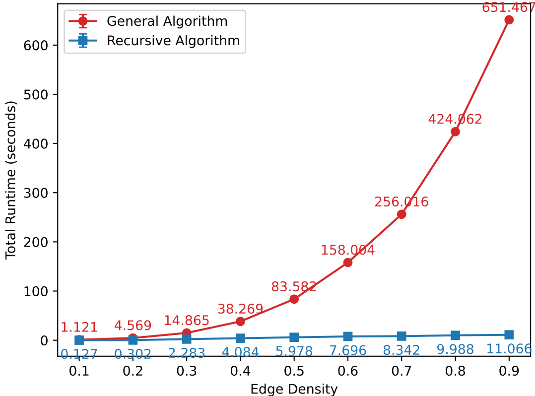
Total Runtime with Basis Tracking (200 realizations per density)
